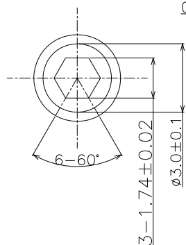
Detail E(2:1) Shaft hole shape and dimension
