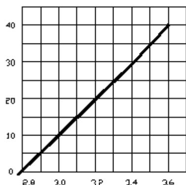
Forward Current vs. Forward Voltage 伏安特性
