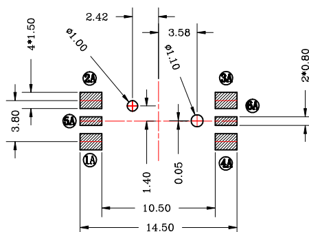
Recommended PCB Layout (Pattern Side) Tolerance: ±0.05mm
