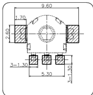
Recommended PCB Layout(Pattern side) tolerance: +/ -0.05mm
