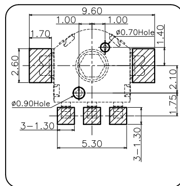
Recommended PCB Layout(Pattern side) tolerance: \pm 0.05\text{mm}
