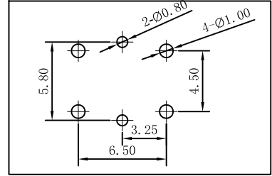
P.C.B layout Pattern Side
