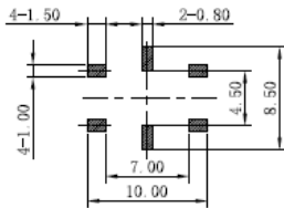
Recommended PCB layout (Pattern Side) Tolerance: ±0.05mm
