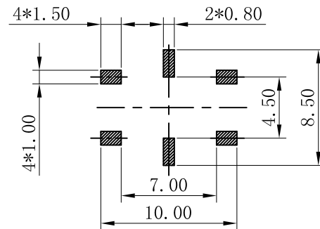
Recommended PCB layout (Pattern Side) Tolerance: ±0.05mm
