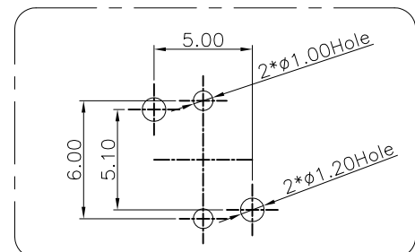
Recommended PCB Layout (Pattern Side) Tolerance: \pm 0.05\text{mm}
