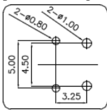
Recommended PCB Layout (Pattern Size/Tolerance: \pm 0.05\text{mm} )
