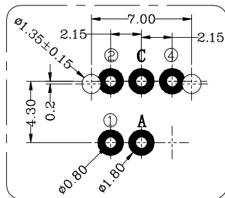
Recommended PCB Layout (Pattern Side) Tolerance: ±0.05mm
