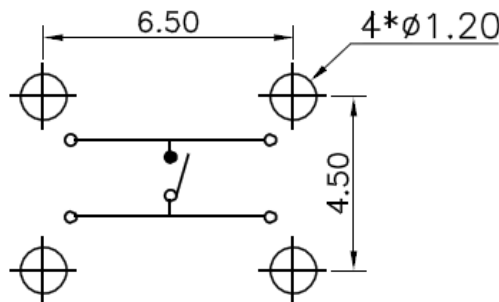
Recommended PCB Layout (Pattern Side) Tolerance: ±0.05mm
