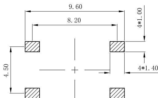
Recommended PCB Layout (Pattern Side) Tolerance: ±0.05mm
