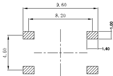
Recommended PCB Layout (Pattern Side) Tolerance: ±0.05mm
